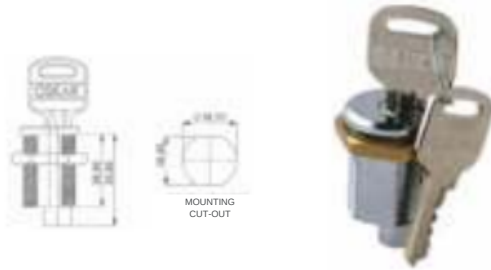
Pedestal Drawer Lock
