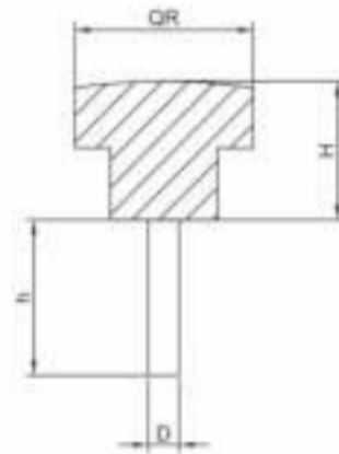
Special plated hexagonal iron insert.
