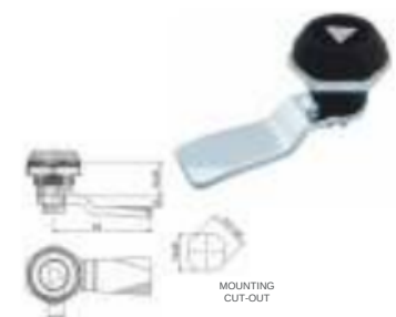
Plastic Spring-Loaded Panel Lock Triangular Insert
