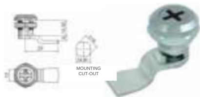
Mini Spring-Loaded Panel Lock Screwdriver Operated
